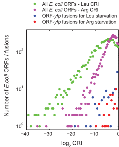
Fig. S7: Histogram of CRI
